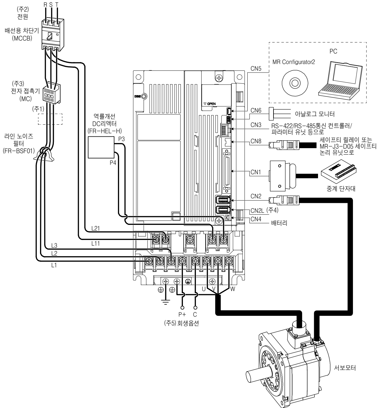
(c) MR-J4-500A4(-RJ)
