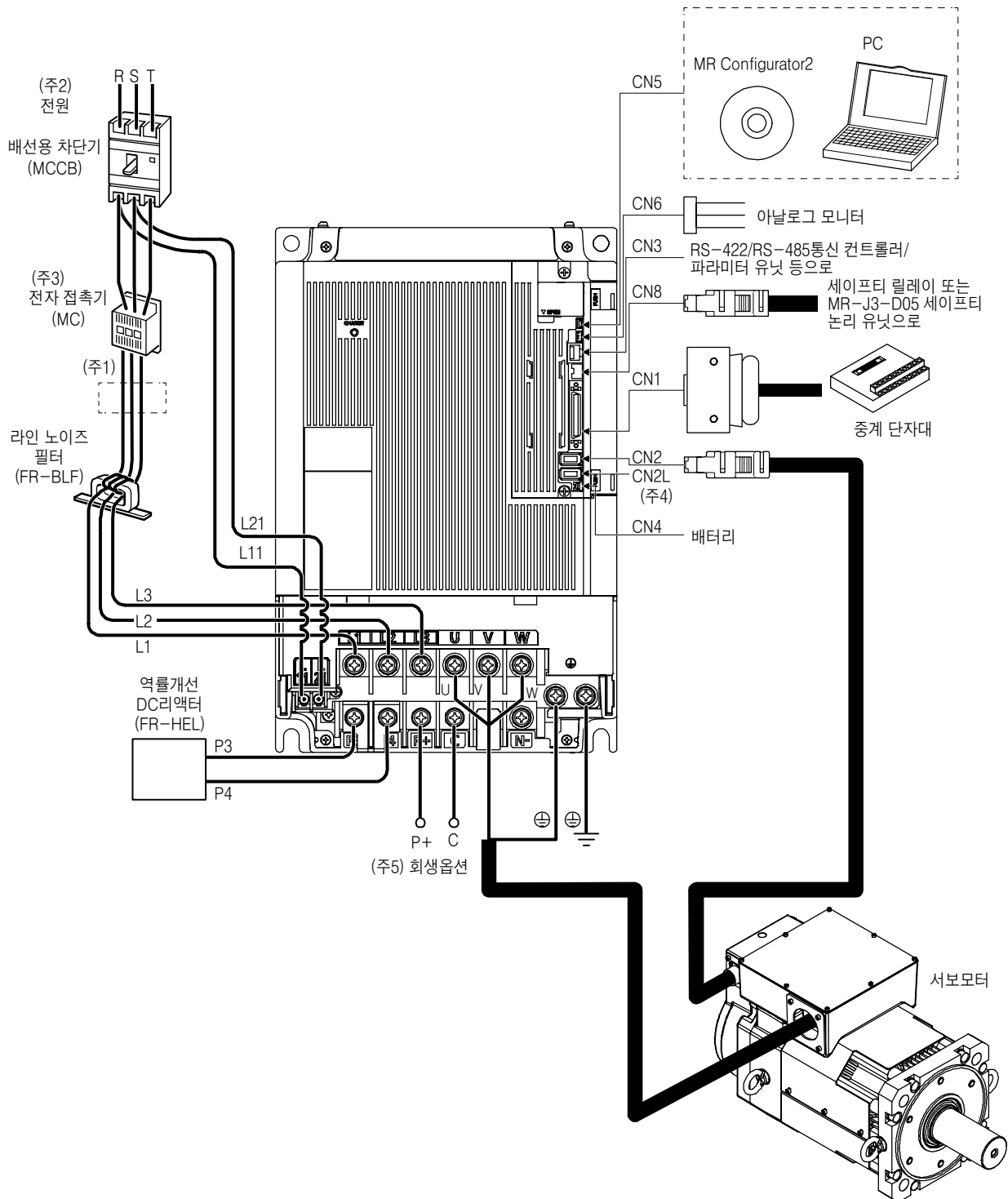
(f) MR-J4-22KA(-RJ)
