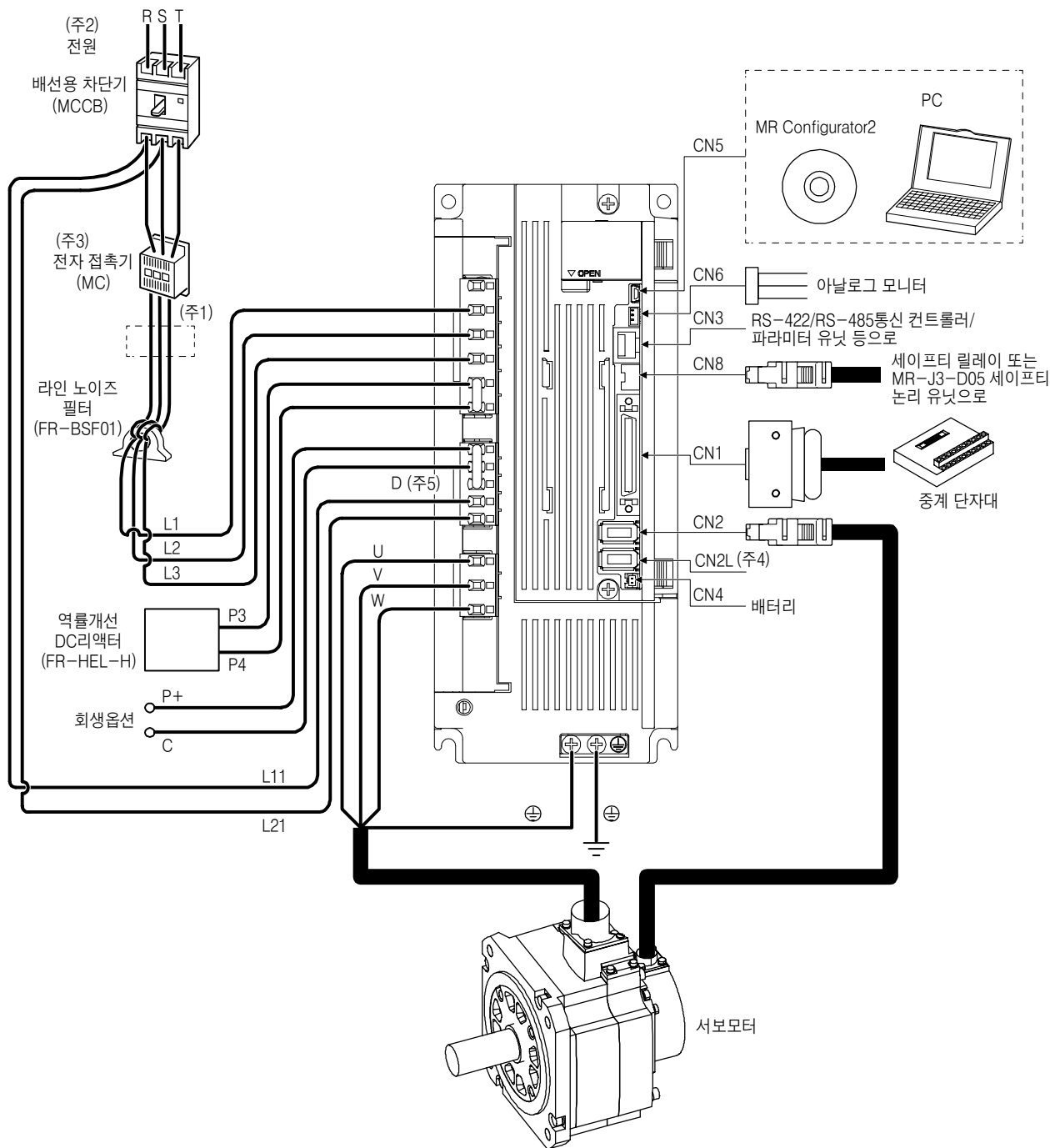
(b) MR-J4-350A4(-RJ)
