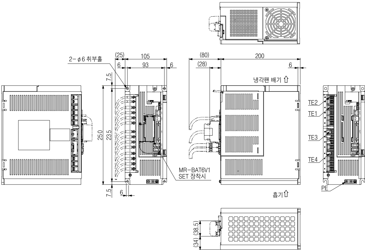
(f) MR-J4-500A(-RJ)
